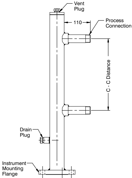
Flanged Chamber - Threaded type
