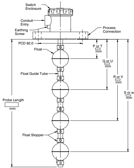
Assembly - Type - 1 ( Flange Connection )
