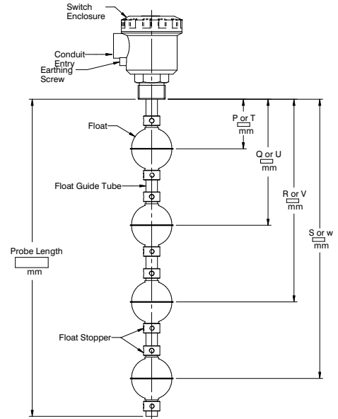
Assembly - Type - 2 ( Threaded Connection )
